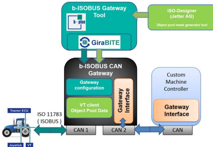
Illustration 2: Workflow configuration
