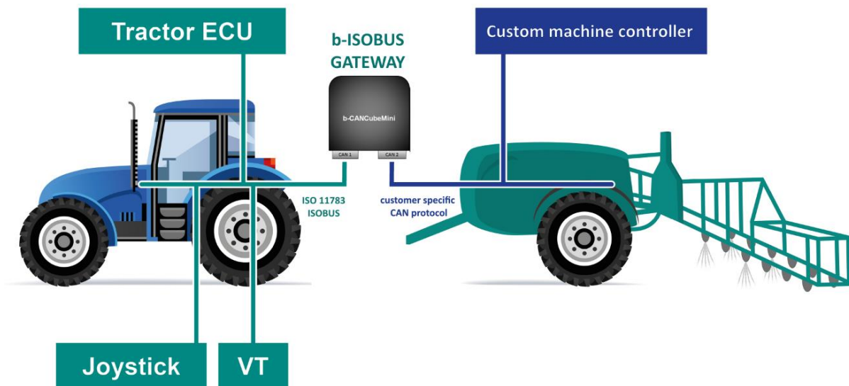
Illustration 1: b-ISOBUS Gateway
